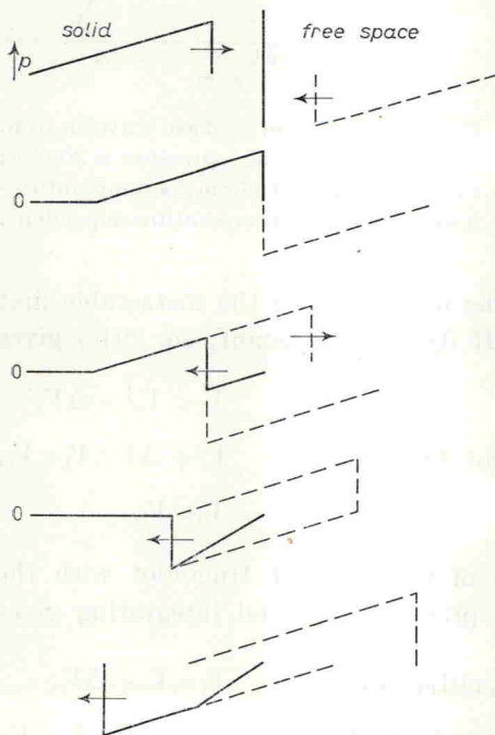
Fig. 25. - Reflection at a free surface, linear waves.
